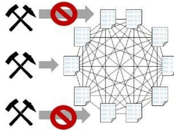
Permissioned Blockchain
