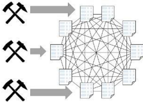
Permissionless Blockchain
